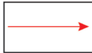
underground river connection 地下河川
