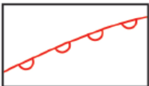
rim of inactive polje ポリエ縁
