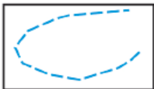
Limit of underground catchment area 地下集水域の限界
