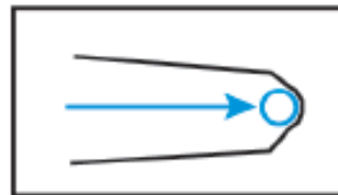
blind valley 盲目谷
