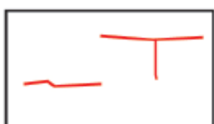
Grikes / Crevasses (岩の)空隙
