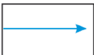
stream (may be drawn ondulated) 流水
