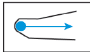
pocket valley 袋谷
